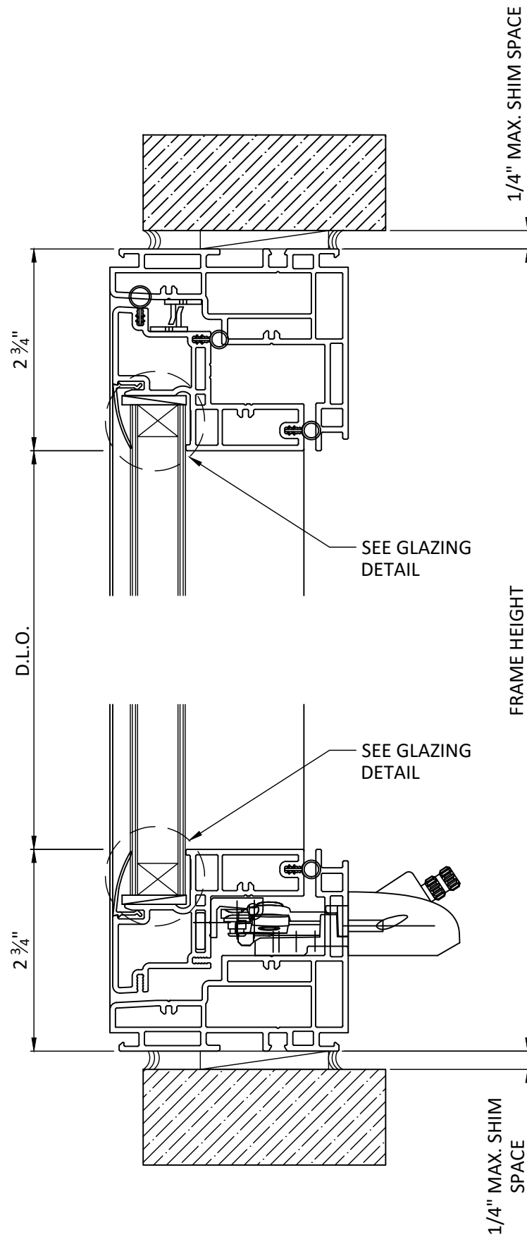
B 3 VERTICAL SECTION AWNING SILL
