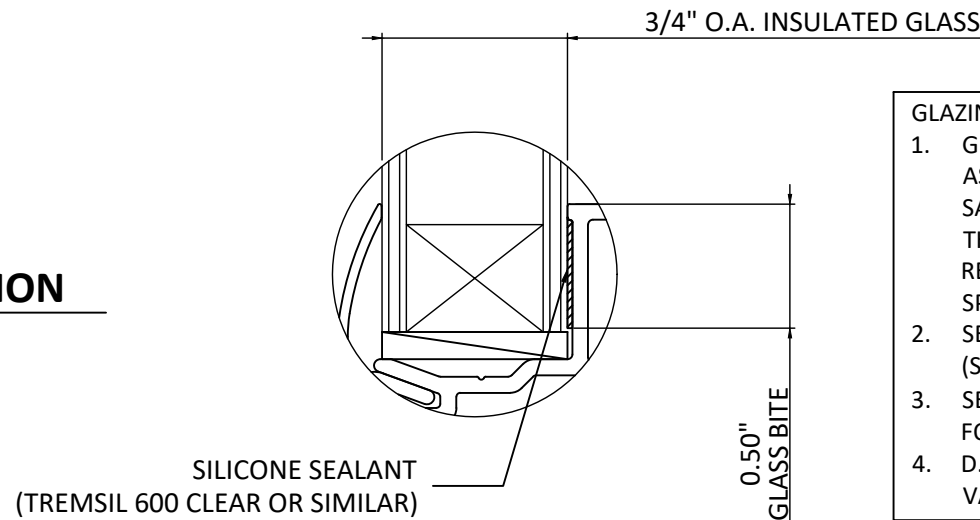
GLAZING DETAIL
